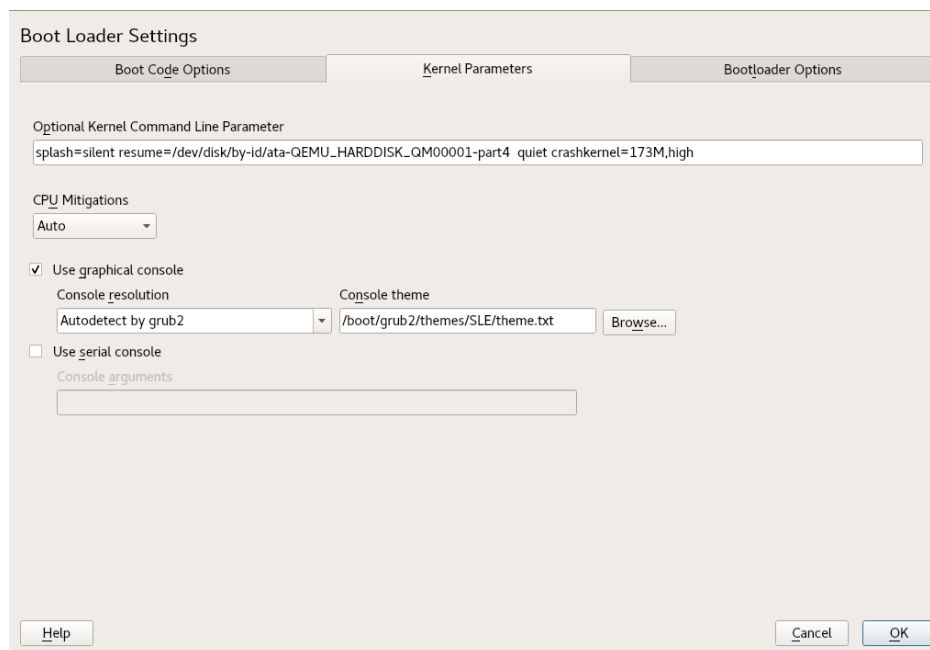
FIGURE 12.5: KERNEL PARAMETERS
