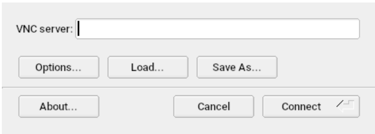
FIGURE 4.1: VNCVIEWER
