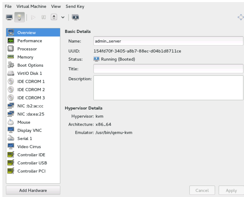
FIGURE 12.1: DETAILS VIEW OF A VM GUEST
