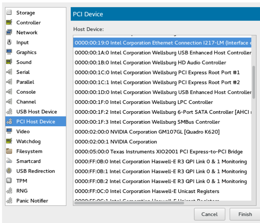
FIGURE 12.15: ADDING A PCI DEVICE
