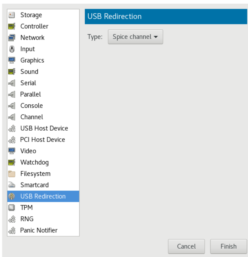
FIGURE 12.14: ADD A NEW USB REDIRECTOR
