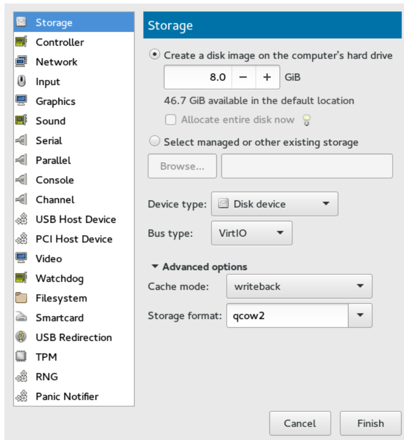
FIGURE 12.9: ADD A NEW STORAGE
